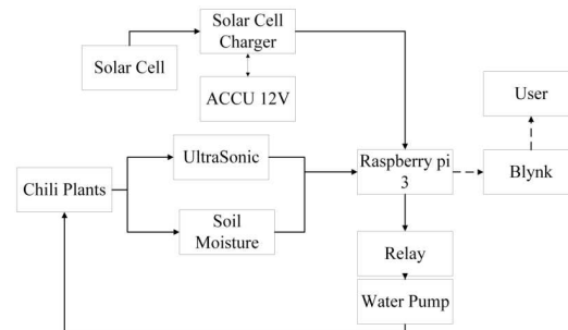
Fig. 1. Block diagram system.
