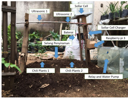
Fig. 7. Hardware implementation.
