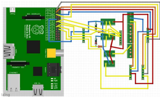
Fig. 2. Monitoring and watering circuit scheme.
