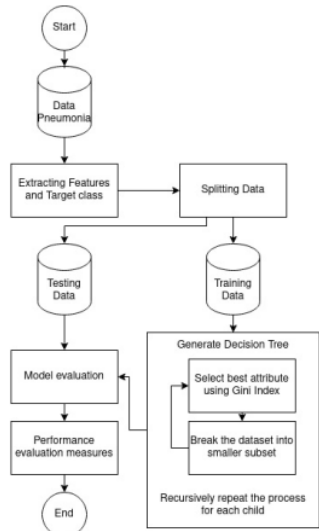
Fig. 2. Flowchart of the CART algorithm to predict pneumonia disease
