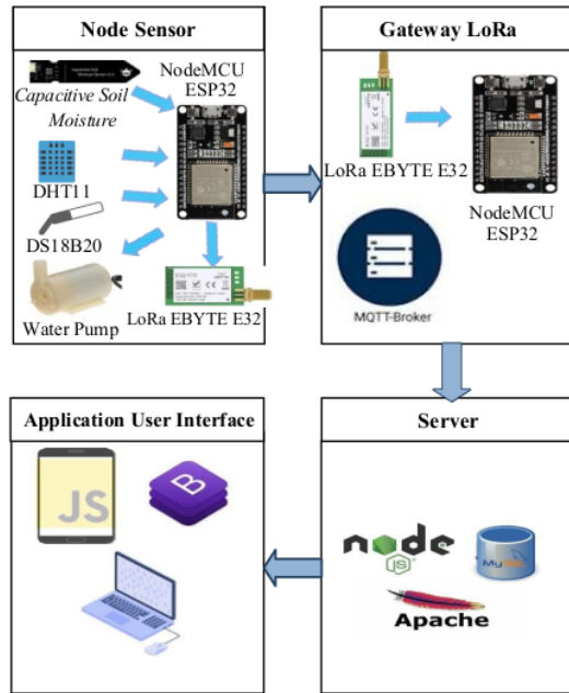
Fig. 1. Designing the overall system.
