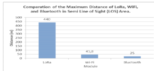
Fig. 3. Comparison graph of the coverage distance of each module in Semi Line of Sight (LOS) area.
