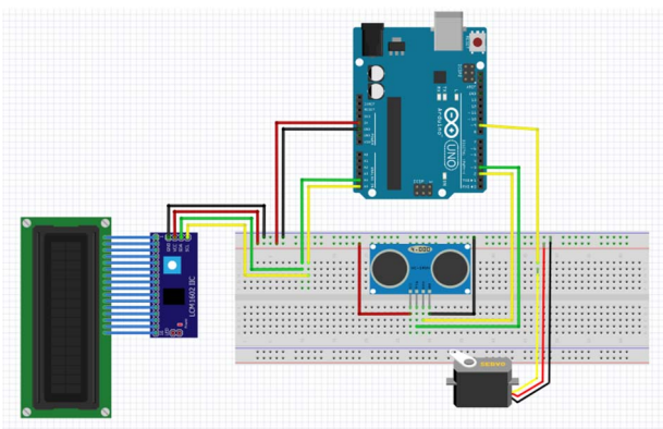
Fig. 5. Schematic electronic circuit detector prototype.
