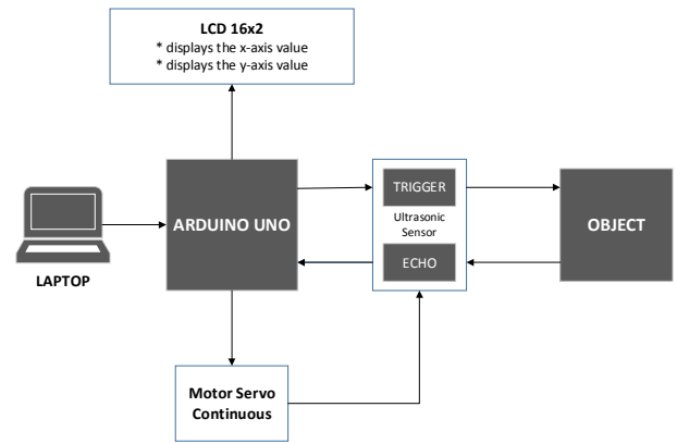
Fig. 2. Prototype's design.
