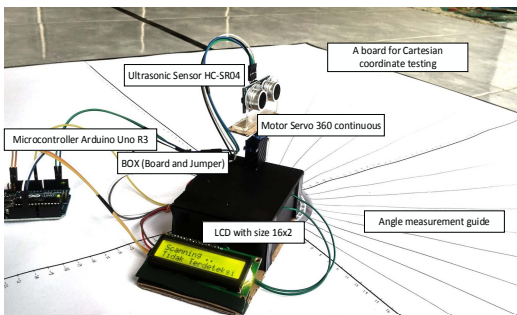
Fig. 7. Prototype of object coordinate detection tool.
