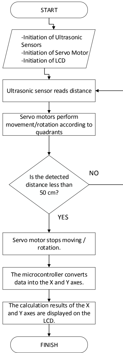
Fig. 6. Flowchart of how the detector prototype works.
