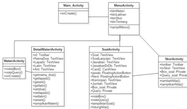
Figure 3. Class Diagram Application
