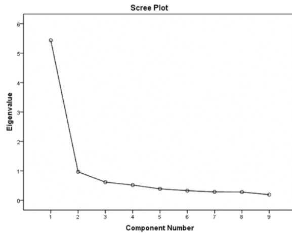
Figure 2. Scree plot
