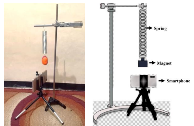
Gbr. 3 Rangkaian Percobaan GHS.
