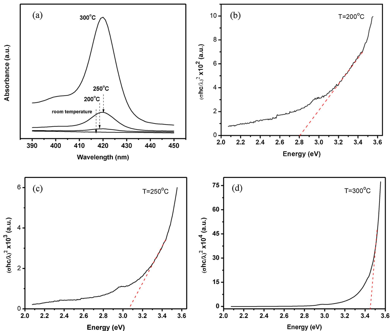
Fig. 2. (a). The absorption spectra of polymer C-Dots from recycled plastic waste, and The estimation of band gap energy polymer C-Dots with heating process at temperature: (b). T = 200 °C, (c). T = 250 °C and (d). T = 300 °C.
