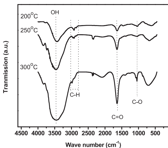
Fig. 5. FTIR spectra of polymer C-Dots from recycled plastic waste.
