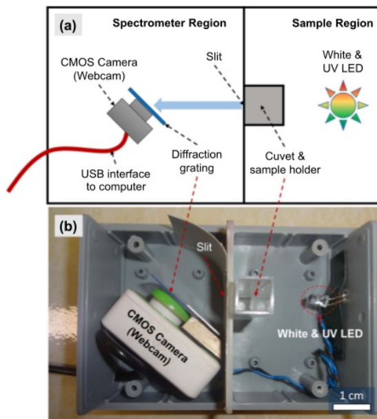
6 Figure 1. (a) Schematic diagram and (b) prototype of the diffraction grating and image processing-based optical spectrometer.
