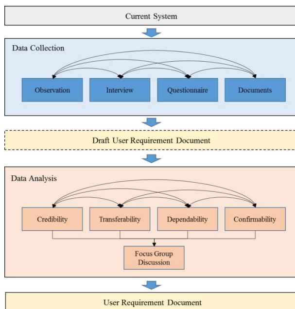
Fig. 1. Concept of needs elicitation in software engineering
